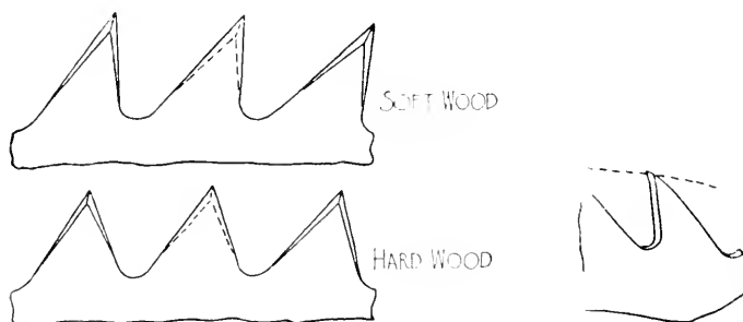
FIG. 180. CIRCULAR CROSSCUT AND RIP-SAW TEETH.
